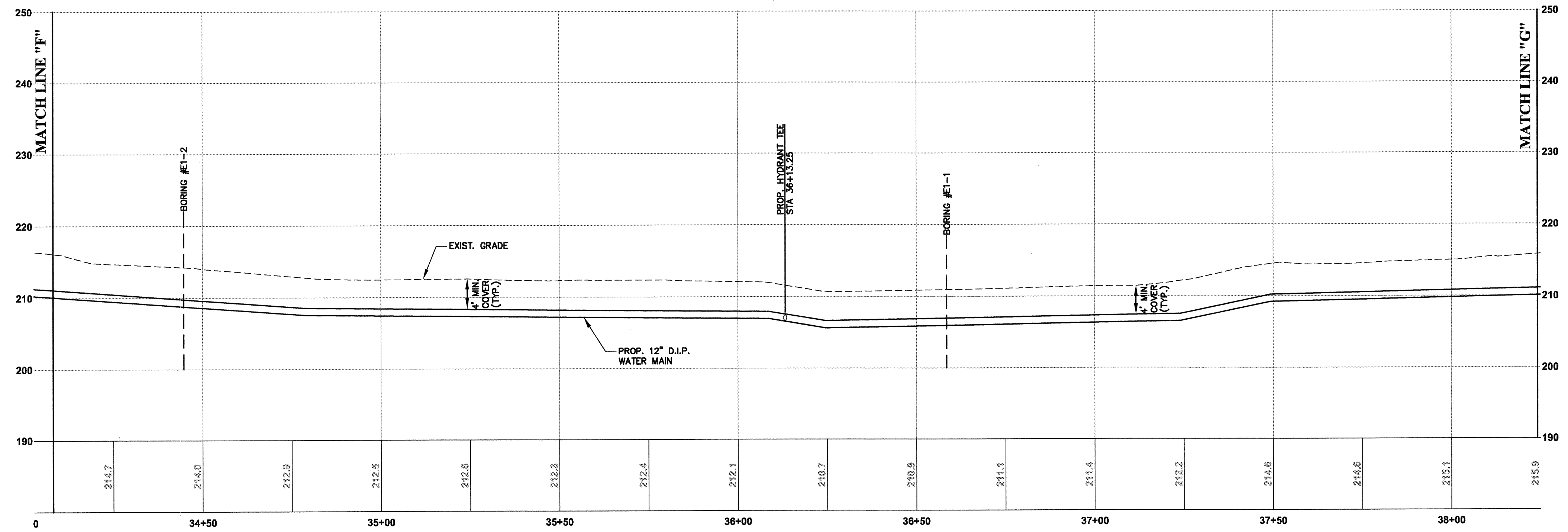
WATER MAIN PROFILE SCALE: HOR. 1" = 20' VER. 1" = 10'
